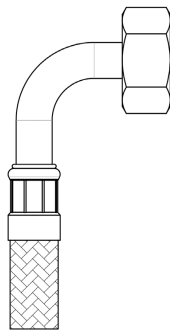
Elbow female
